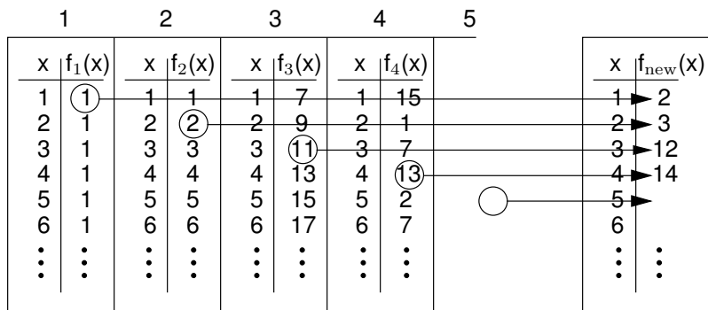
Figure 17.6 Illustration for the argument that the number of integer functions is uncountable.
