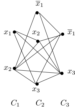
Figure 17.4 The graph generated from boolean expression B = (x_1 + x_2) \cdot (\bar{x}_1 + x_2 + x_3) \cdot (\bar{x}_1 + x_3) . Literals from the first clause are labeled C1 , and literals from the second clause are labeled C2 . There is an edge between every two pairs of vertices except when both vertices represent instances of literals from the same clause, or a negation of the same variable. Thus, the vertex labeled C1 : y_1 does not connect to the vertex labeled C1 : y_2 (because they are literals in the same clause) or the vertex labeled C2 : \bar{y}_1 (because they are opposite values for the same variable).
